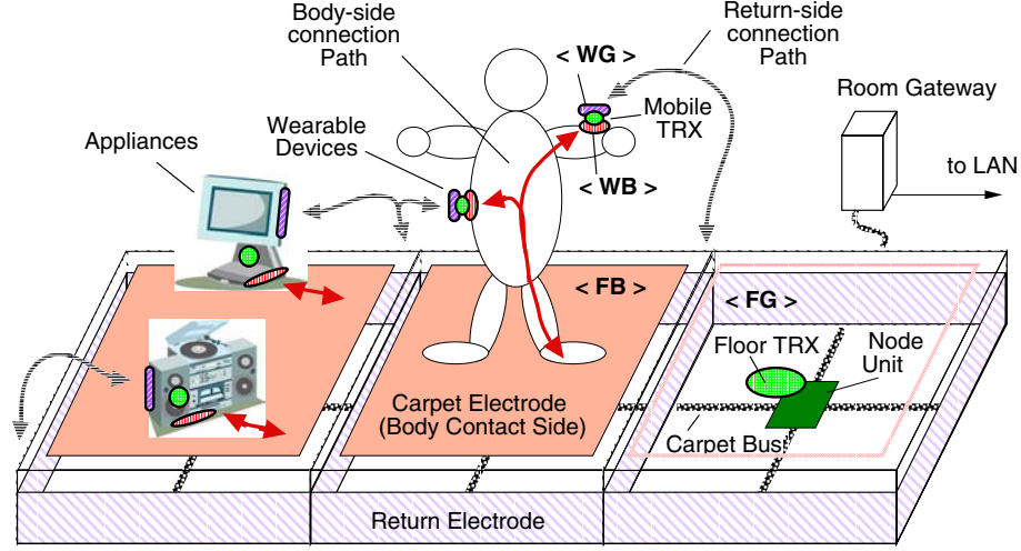
Fig. 1. System architecture. Each carpet-unit works as a network cell.
