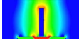
(c) Electric field distribution (floor and wearable device)
