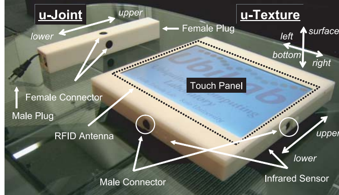
Fig. 3. A u-Texture (right) and a u-Joint (left)
