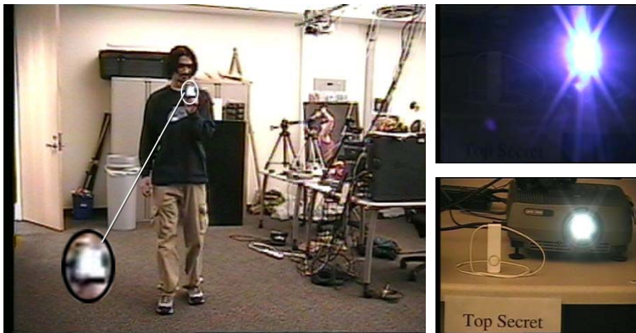
Figure 5. Left is a camera phone being neutralized by our system (notice the neutralizing light beam over the lens). Top right is the camera view neutralized by the system and bottom right is the camera view when the camera is permitted to capture.
