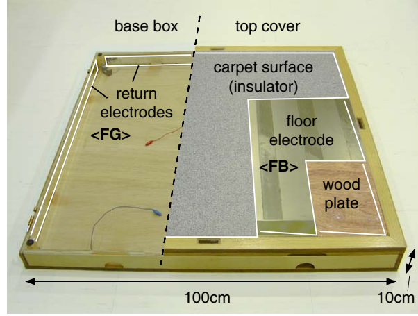
Fig. 5. Carpet Box (left) Return electrode strips / (right) Floor top electrode (covered)
